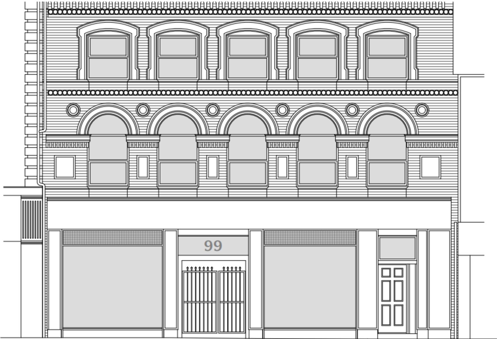
Existing Front (West) Elevation from High Street
