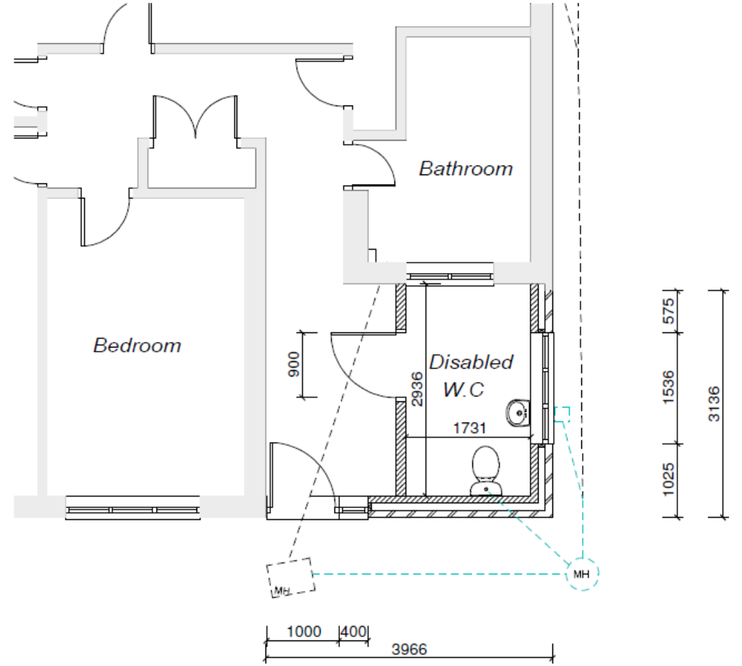
Proposed Layout 1:50
