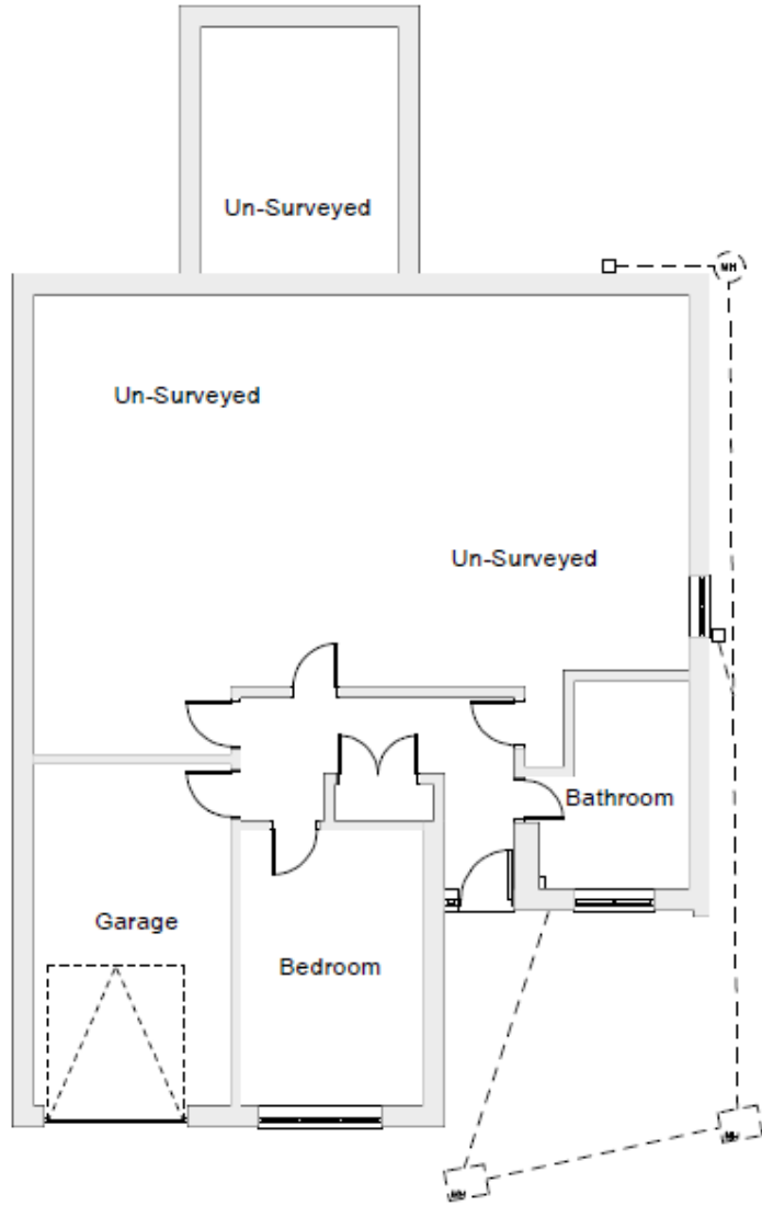
Existing Layout 1:100
