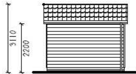
East Elevation 1:100
