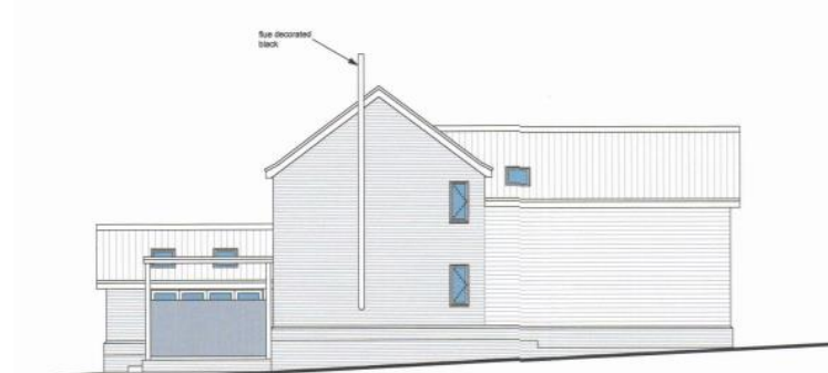
EAST ELEVATION
