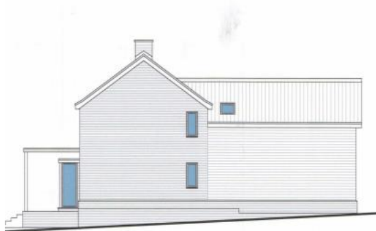
EAST ELEVATION
