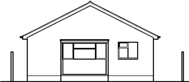
Existing Rear Elevation Scale: 1/100
