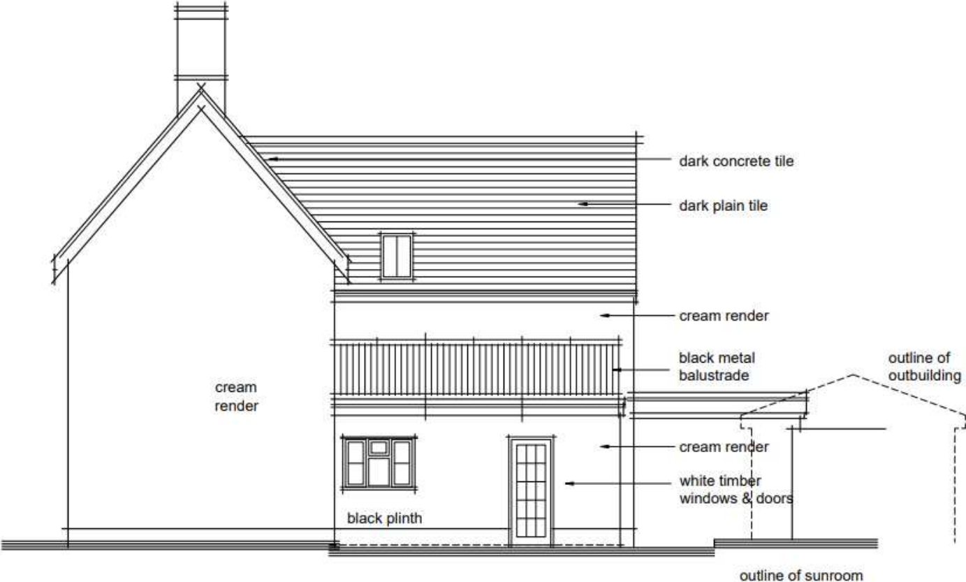
Side Elevation - Existing
