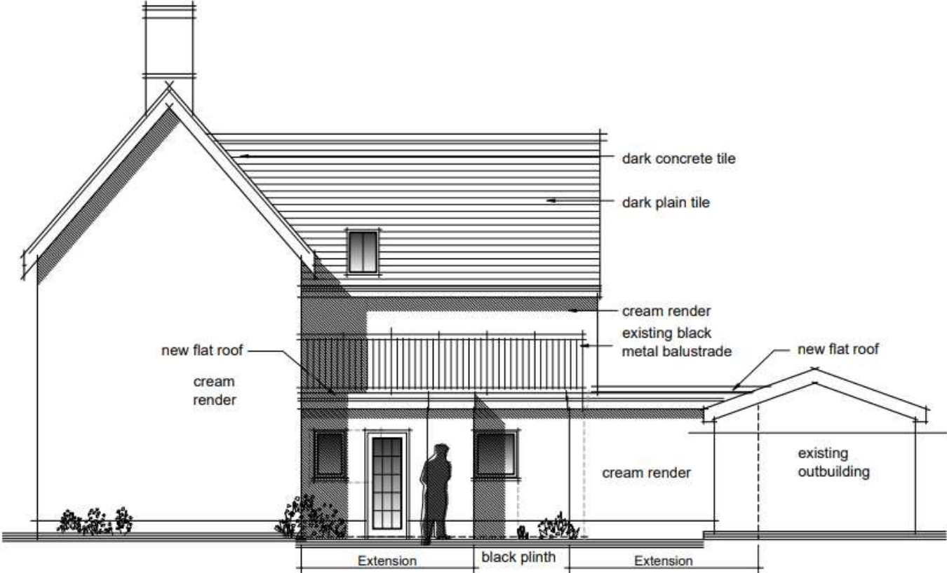
Side Elevation - Proposed
