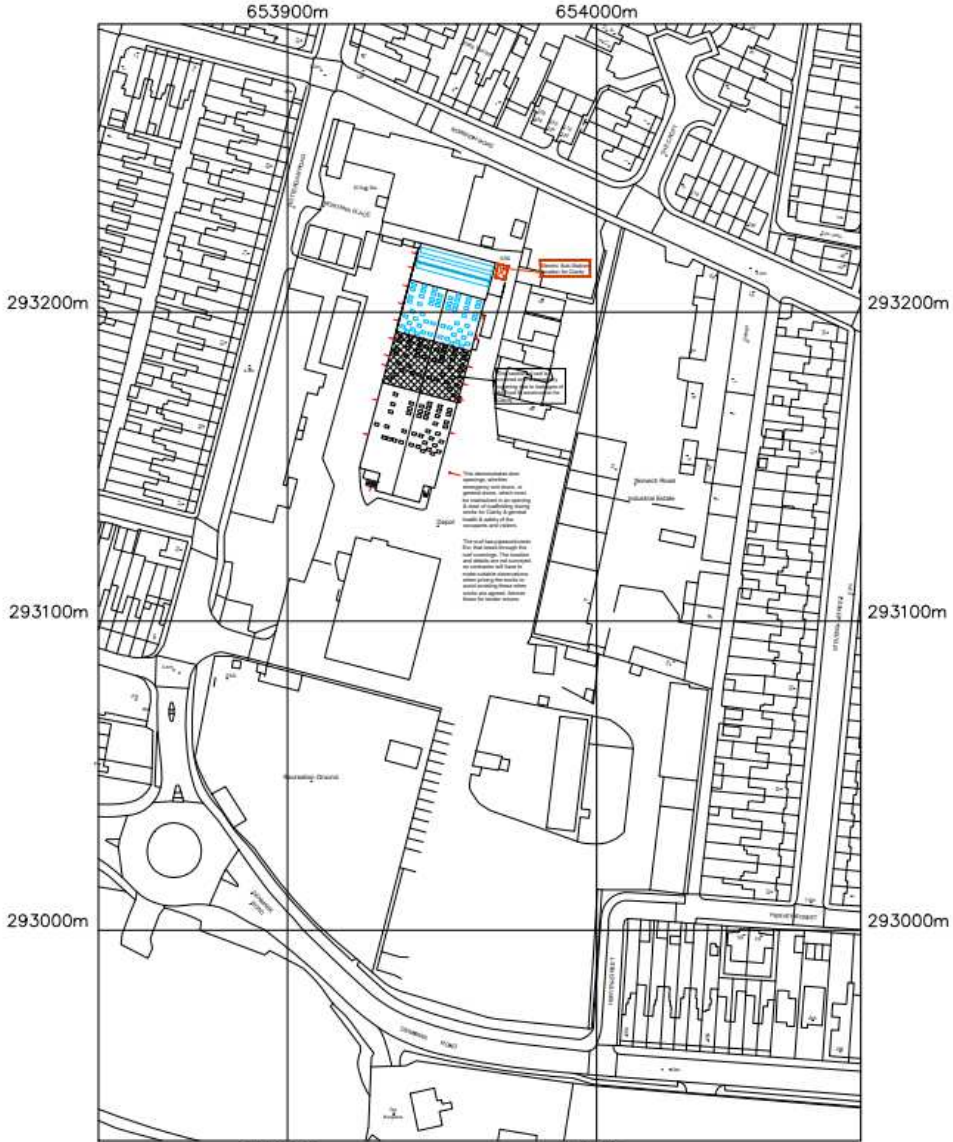
EXISTING BLOCK PLAN
